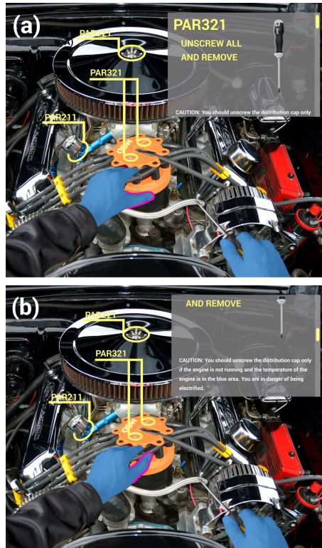
Application scenario and envisioned interaction examples. A mechanic who is following AR instructions (a) can swipe on the nearby cable to (b) scroll down the instructions view.
