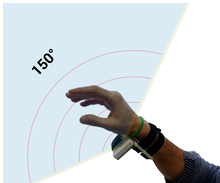
Figure 1: We used a wrist-mounted Google Soli for sensing micro-gestures on physical objects.
