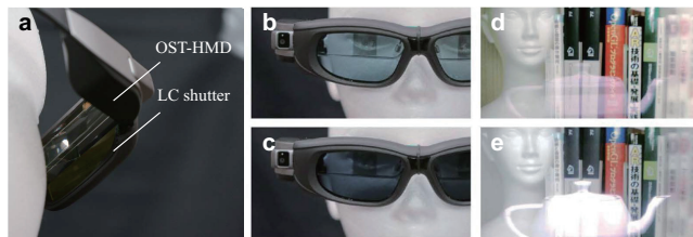
Figure 1: Our prototype OST-HMD (a-c) and conceptual images captured with a camera with automatic gain control (d, e). Our OST-HMD gradually reduces LC transparency (b to c) and increases the perceived brightness of the virtual content (Utah teapot) without making the user aware of real scene dimming (d to e).
